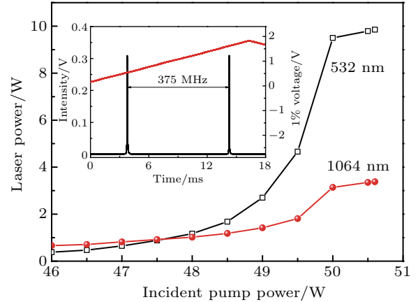
Fig. 2. Output powers of 1.06 \mu\text{m} and 532 nm lasers versus incident pump power. Inset: transmitted intensity of F–P 1 interferometer.
