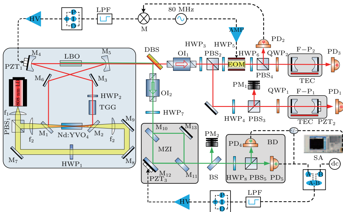
Fig. 1. Experimental setup of high power cw single-frequency dual-wavelength laser and stabilization system. LPF: low pass filter; M: mixer; HV: high voltage amplifier; AMP: power amplifier; dc: direct current source; OI: optical isolator; EOM: electro-optic modulator; PID: proportional-integral-derivative amplifier; A and B: negative power combiner; +/−: positive/negative power combiner; SA: spectrum analyzer.
