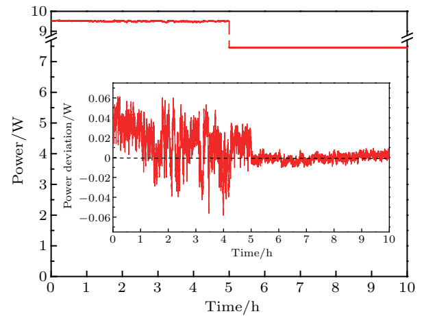
Fig. 7. Power fluctuation of the 532 nm laser before MZI (0–5 h) and output from a locked MZI (5–10 h).
