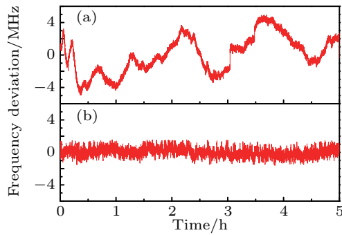
Fig. 3. Frequency drift of (a) free running laser and (b) stabilized laser in 5 h.
