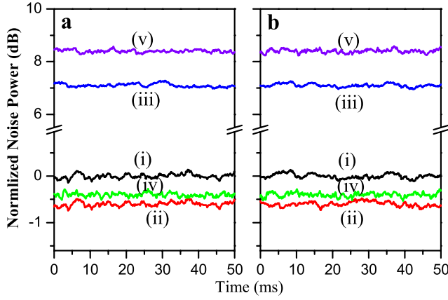
FIG. 4 (color online). The correlation variance of the superactivated EPR entanglement measured at the sideband mode of 2 MHz. (a) \langle \delta^2(\hat{x}_{b_1} + \hat{x}_{b_{4'}}) \rangle , (b) \langle \delta^2(\hat{p}_{b_1} - \hat{p}_{b_{4'}}) \rangle . (i) The QNL; (ii)[(iv)] The correlation noise power with the help of station B, C and D for \langle \delta^2 \hat{x}_{v_1} \rangle = \langle \delta^2 \hat{p}_{v_1} \rangle = 2.70 \pm 0.01 [4.70 \pm 0.02] ; (iii)[(v)] The correlation noise power without the help of stations B, C, and D for \langle \delta^2 \hat{x}_{v_1} \rangle = \langle \delta^2 \hat{p}_{v_1} \rangle = 2.70 \pm 0.01 [4.70 \pm 0.02] .
