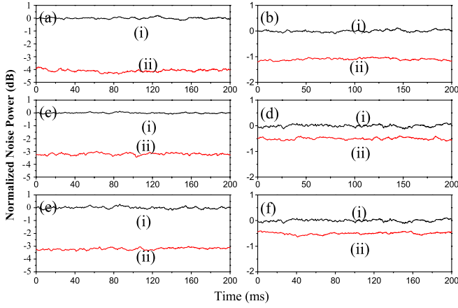
FIG. 3 (color online). The measured correlation variance of three-color entangled states at 2 MHz. a, \langle \delta^2(X_3 - X_4) \rangle , b, \langle \delta^2(g_1^{\text{opt}}Y_3 + Y_3 + Y_4) \rangle , c, \langle \delta^2(X_2 - X_4) \rangle , d, \langle \delta^2(Y_2 + g_2^{\text{opt}}Y_3 + Y_4) \rangle , e, \langle \delta^2(X_2 - X_3) \rangle , f, \langle \delta^2(Y_2 + Y_3 + g_3^{\text{opt}}Y_4) \rangle . (i) The QNL; (ii) The correlation noise power. The resolution and video bandwidths of spectrum analyzer are 30 kHz and 100 Hz, respectively.
