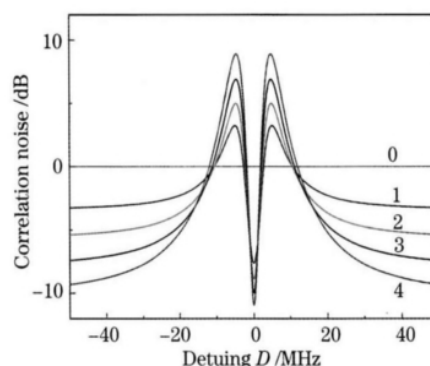
图 2 NOPA 输出场的关联噪声随腔失谐的变化 Fig. 2 Dependence of correlation noise of output field of NOPA on detuning of the cavity
