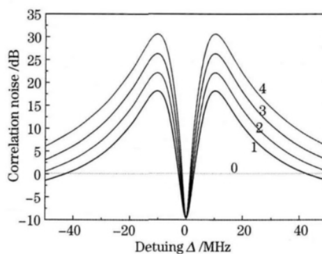
图6 NOPA 输出场关联噪声随反关联分量的额外噪声的变化 Fig. 6 Dependence of correlation noise of output field of NOPA on extra noise in anti-correlation quadrature
