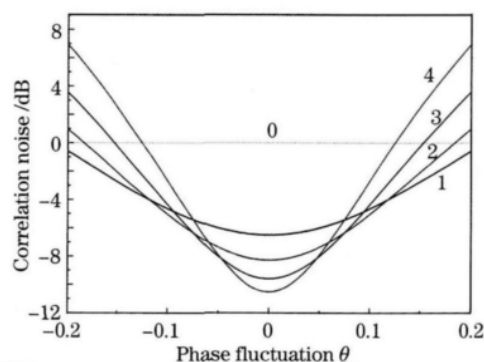
图5 输出场关联噪声随相位波动的变化 Fig. 5 Dependence of correlation noise of output field of NOPA on phase fluctuation
