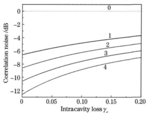
图3 NOPA 输出场关联噪声随内腔损耗的变化 Fig. 3 Dependence of correlation noise of output field of NOPA on intracavity loss
