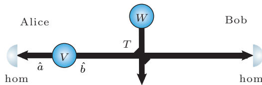
Fig. 1. (color online) Schematic plot of a symmetric two-mode Gaussian entangled state distributed between Alice and Bob through a lossy channel with excess noise. The transmission efficiency of quantum channel is modeled by a beam splitter with transmission T . Excess noise in the channel is modeled by an environmental thermal state \rho_E with variance W . Alice and Bob perform homodyne (hom) detection on the mode they hold, respectively.
