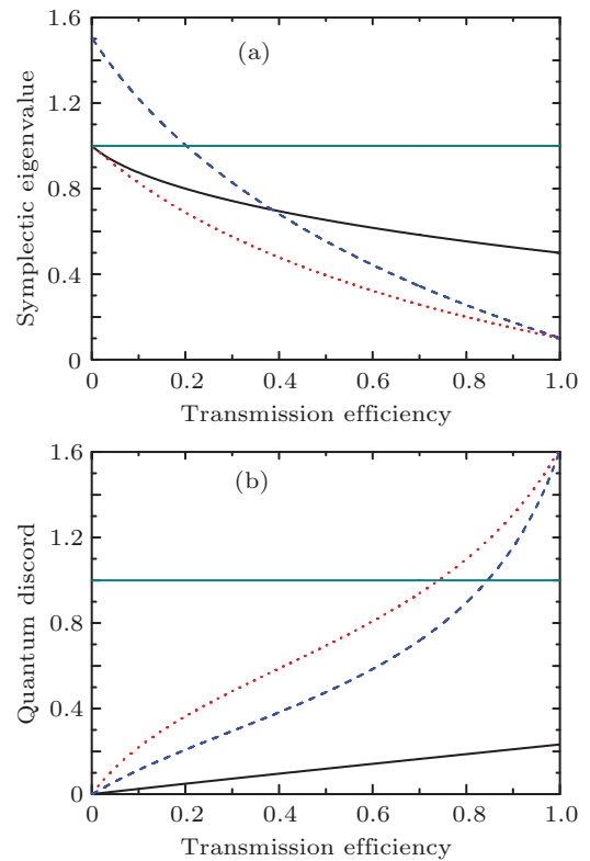
Fig. 2. (color online) (a) Symplectic eigenvalues with different variances of resource state and (b) Gaussian quantum discords with different variances of resource state. Dotted (red) and solid (black) lines in panels (a) and (b) correspond to r = 1.15 and r = 0.35 with W = 1 , respectively. Dashed (blue) lines in panels (a) and (b) correspond to r = 1.15 with W = 1.5 .
