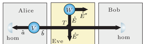
Fig. 3. (color online) Schematic of the QKD scheme with an EPR entangled state. The transmission efficiency of the quantum channel is modeled by a beam splitter with transmission T . Eve performs an entangling cloner attack, where the variance of the EPR state is W . Alice and Bob perform homodyne (hom) detection on the mode they hold, respectively.
