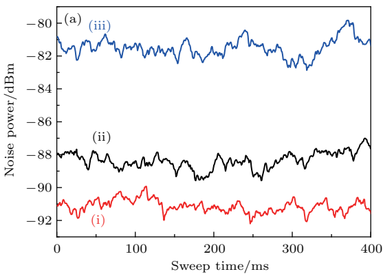
Fig. 4. Normalized noise power spectra of squeezed light at 1.34 \mu\text{m} . Curve i is squeezed noise, curve ii is SNL, curve iii is anti-squeezed noise.
