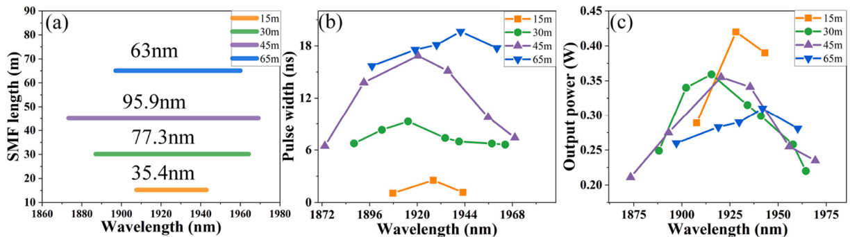
Fig. 5. The wavelength tunable range under different SMF lengths. Comparison of the (b) pulse width and (c) output power of fiber laser with different fiber lengths.
