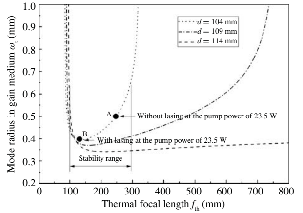
Fig. 2. Beam radius of fundamental wave in gain medium versus thermal focal length f_{th} for three different distances d between M_3 and M_4 .
