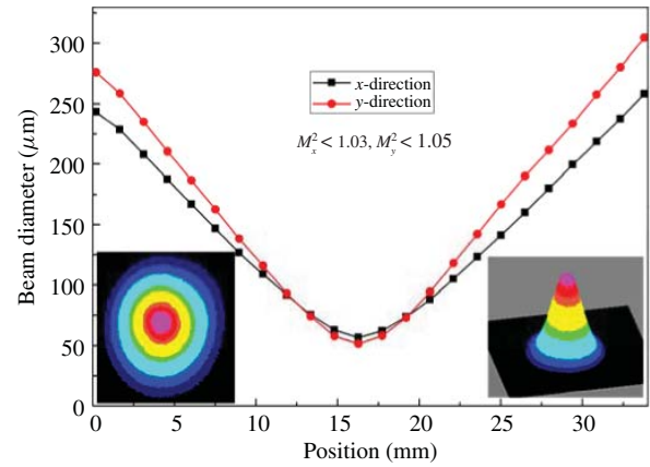
Fig. 6. Measurement of beam quality, spatial beam profile, and intensity distribution.
