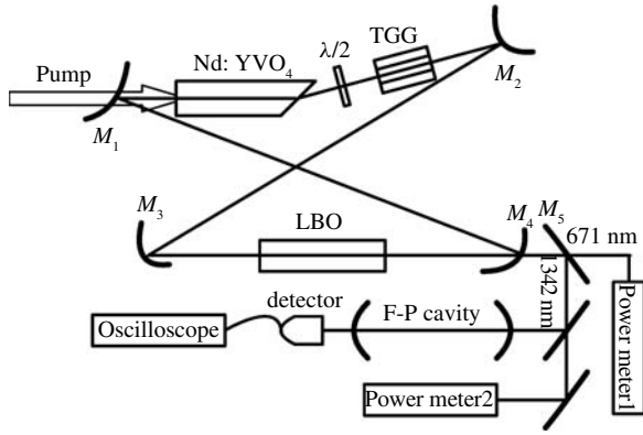
Fig. 3. Experimental schematic of the high-power single-frequency red laser. \lambda/2 : half wave plate. TGG: terbium gallium garnet.
