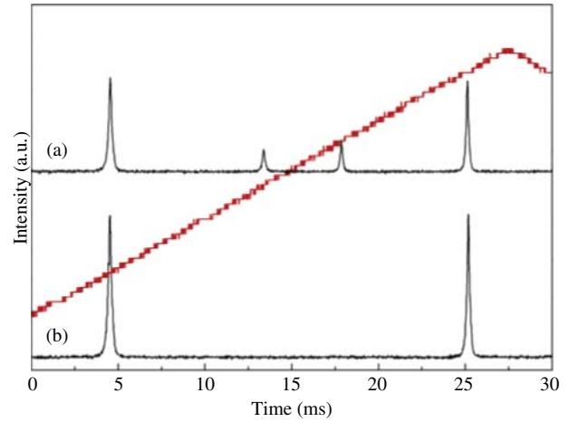
Fig. 4. Scanning confocal Fabry-Perot spectra of the fundamental wave, confirming the single-frequency operation (a) without intracavity nonlinear process and (b) with intracavity nonlinear process. The scanning ramp voltage is also shown.
