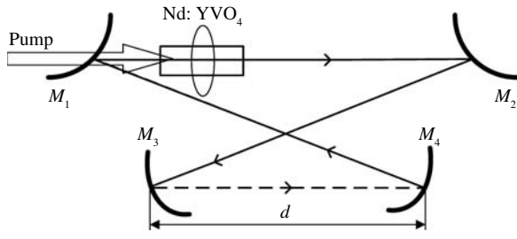
Fig. 1. Configuration of the laser resonator.
