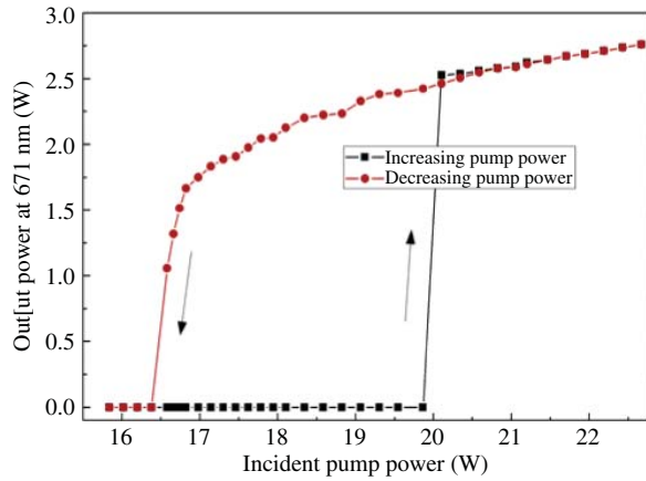
Fig. 5. Output power of the harmonic wave versus incident pump power for increasing and decreasing pump power.
