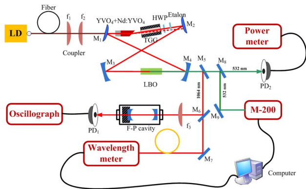
Fig. 1. (Color online) Experimental setup of the tunable single-frequency green laser.
