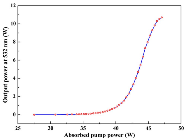
Fig. 2. (Color online) Output power of the single-frequency green laser versus pump power.
