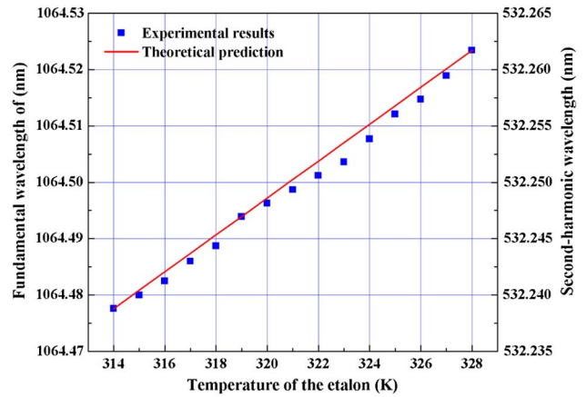
Fig. 6. (Color online) Wavelength of the fundamental wave dependent on the temperature of the quartz etalon.
