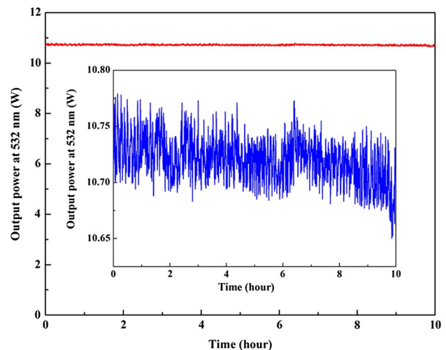
Fig. 3. (Color online) Power stability of the green laser in 10 h.
