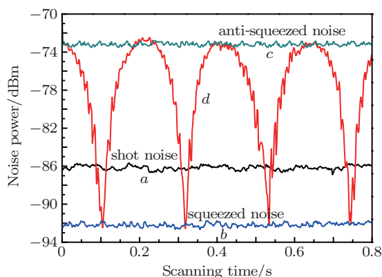
Fig. 3. (color online) Measured quantum noise levels of the squeezed vacuum at a pump power of 260 mW as the local oscillator phase is scanned. The noise level is measured with a spectrum analyzer at the Fourier sideband frequency of 2 MHz, with a resolution bandwidth of 30 kHz and a video bandwidth of 100 Hz. Trace a corresponds to the SNL. Traces b and c represent squeezed and anti-squeezed noise. Trace d shows the quantum fluctuations depending on the local oscillator phase, when the squeezed vacuum is injected.
