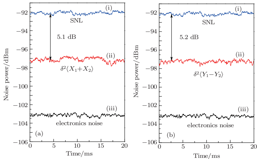
Fig. 4. (color online) The measured entangled light noise powers of (a) amplitude sum and (b) phase difference at 2 MHz: (i) shot noise limit, (ii) correlation noise, (iii) electronics noise. The RBW and VBW of spectrum analyzer are 39 kHz and 30 Hz, respectively.
