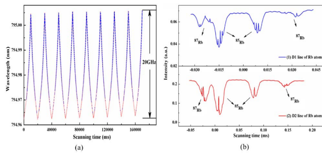
Fig. 6. (a) Continuously frequency tuning of the Ti:sapphire laser. (b) Saturation absorption spectroscopy of the Rb atoms. (1) D 1 line and (2) D 2 line.
