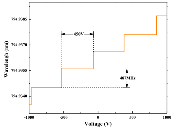
Fig. 4. Variation of the output wavelength of the Ti:sapphire laser with varied high-voltage dc signal applied to the etalon.
