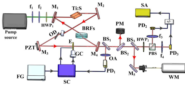
Fig. 1. Experimental setup of the continuous frequency-tuning laser. HWP 1 and HWP 2 , half-wave-plate; Ti:S, Ti:sapphire; OD, optical diode; BRFs, birefringent filters; E, etalon; GC, galvanometer scanner; FG, function generator; SC, servo controller; OA, optical attenuator; PD 1 -PD 3 , photodetectors; BS 1 -BS 3 , beam splitter; PBS, polarization beam splitter; PM, power meter; WM, wavelength meter; SA, spectral analyzer.
