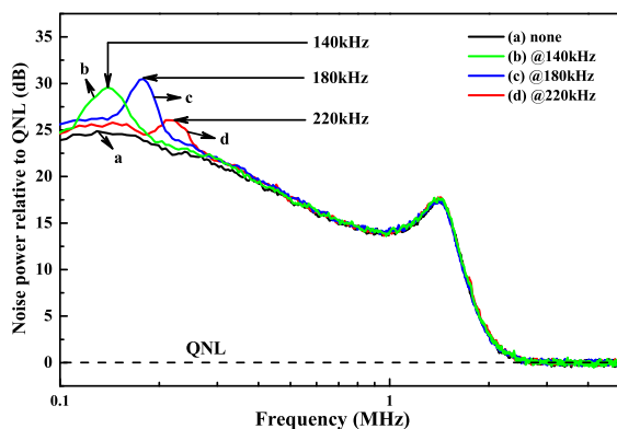
Fig. 7. Intensity noise of the Ti:sapphire laser at different modulation frequencies. (a) Without modulation signal, (b) at 140 kHz, (c) at 180 kHz, and (d) at 220 kHz.
