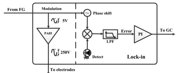
Fig. 5. Schematic of the servo controller.
