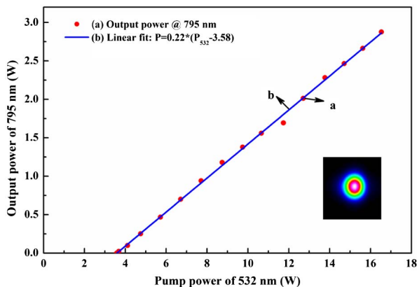
Fig. 3. Output power of Ti:sapphire laser at 795 nm versus the pump power. Inset: spatial beam profile of output laser.
