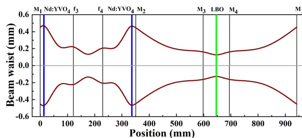
Fig. 2. Beam diameter inside the optimized oscillator.
