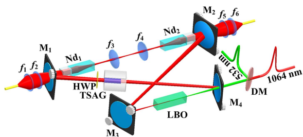
Fig. 1. Schematic of the experimental setup. TSAG, terbitium scandium aluminum garnet; Nd_{1-2} , YVO_4/Nd:YVO_4 ; LBO, lithium triborate; HWP, half-wave plate; DM, dichroic mirror; f_{1-6} , lens.
