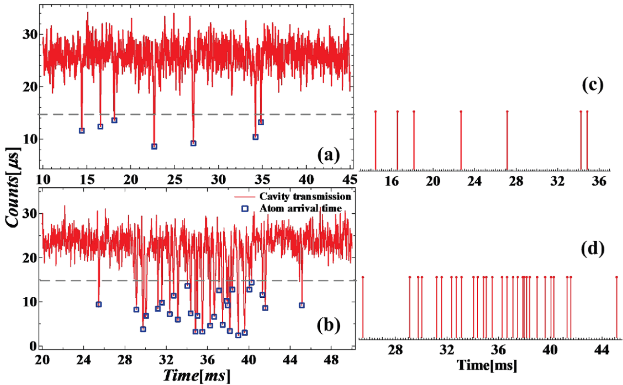
Figure 2. Cavity emission signals from two cold atom samples detected by the SPCM: (a) without PGC and (b) with PGC. The signals from the atoms increased after PGC, and their arrival time was delayed when other conditions were the same. The red curve is the direct output from the SPCM, and a sudden drop in cavity emission (blue squares) corresponded to the arrival of an atom in the cavity. Figures 2(c) and (d), corresponding to figures 2(a) and (b), respectively, illustrate the arrival times of the atoms more clearly.
