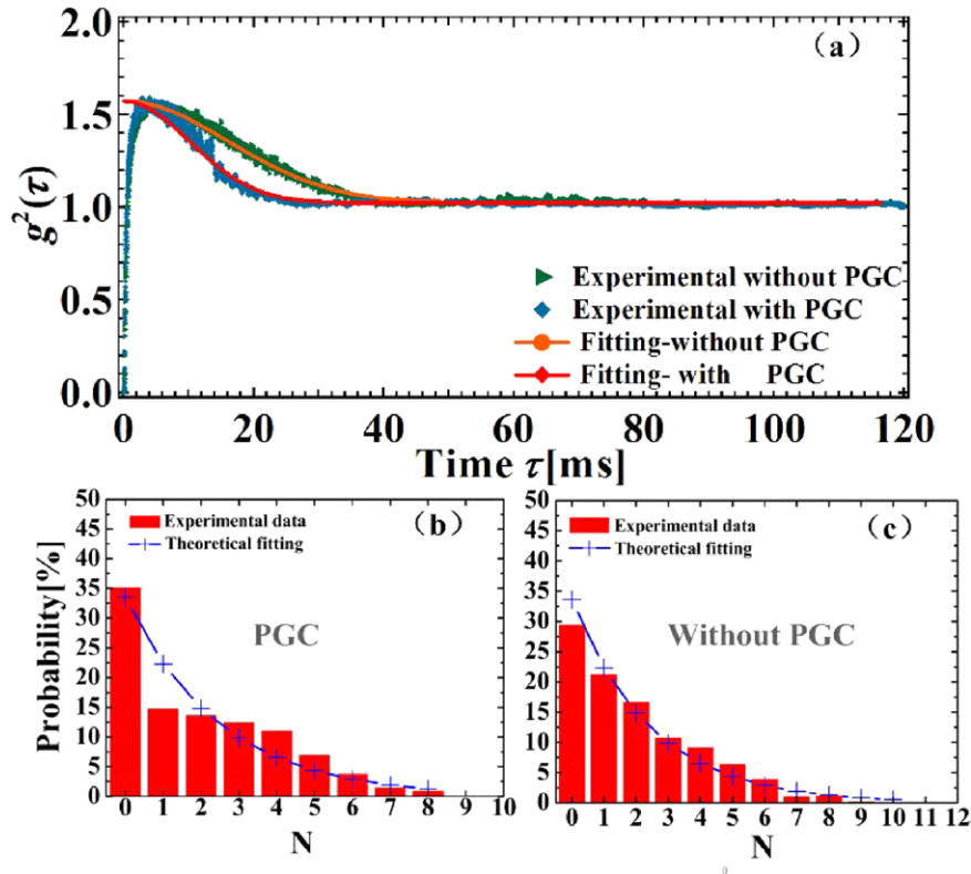
Figure 4. (a) Second-order correlation functions of truly thermal atomic beams. The green triangle line is without PGC, the blue diamond line with PGC. The orange and red lines are the corresponding curves fitted according to the theory of multimode thermal field coherence. (b),(c) The probability distribution of the number of events N for a time interval of T = 20.7 ms after PGC (b), and T = 28.5 ms without PGC (c). The crosses (+) indicate a Bose distribution with the same mean value of \langle n \rangle = 1.97 .
