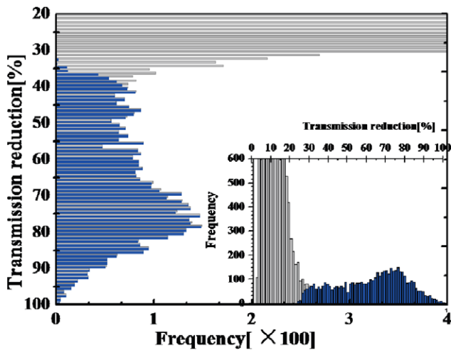
Figure 3. Distribution of measured cavity transmission reduction magnitudes. The black bars indicate the extracted atom signal from setting twice the threshold, and the blue bars are for four times the threshold. The inset illustration shows the enlarged view. It proved that four times the standard deviation of the photon shot noise as the threshold was better for recognizing a real atom event than twice the standard deviation.
