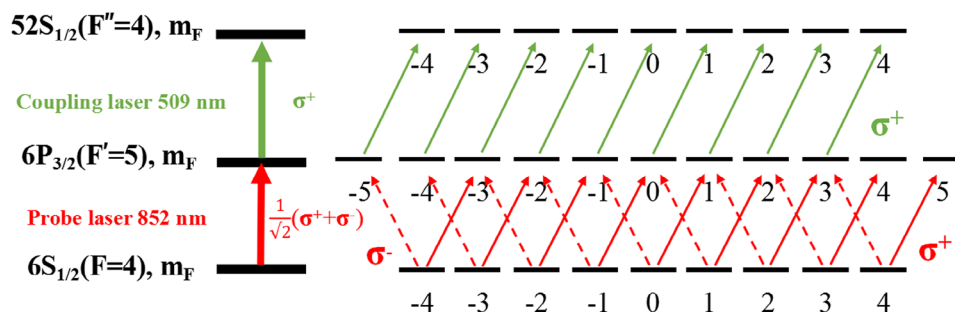
Figure 1. Schematic of the Rydberg ladder-type three level system ( 6S_{1/2} - 6P_{3/2} - 52S_{1/2} ). The probe beam is linearly polarized and the coupling beam is circularly polarized. The 852 nm probe beam is locked to the 6S_{1/2} ( F = 4 )- 6P_{3/2} ( F' = 5 ) transition, and the 509 nm coupling beam frequency is scanned over the 6P_{3/2} ( F' = 5 )- 52S_{1/2} . The 509 nm right circularly polarized beam passes through Cs vapor, causing the non-uniform distribution on the Zeeman states, and the Cs vapor turn into an anisotropic medium, the 852-nm linearly polarized beam can be regarded as a combination of \sigma^+ and \sigma^- , and when passing through the anisotropic medium, the refractive indices of the left and right polarization components are different, so that the 852 nm polarization changes and TCPS is obtained by using a balanced photodetector.
