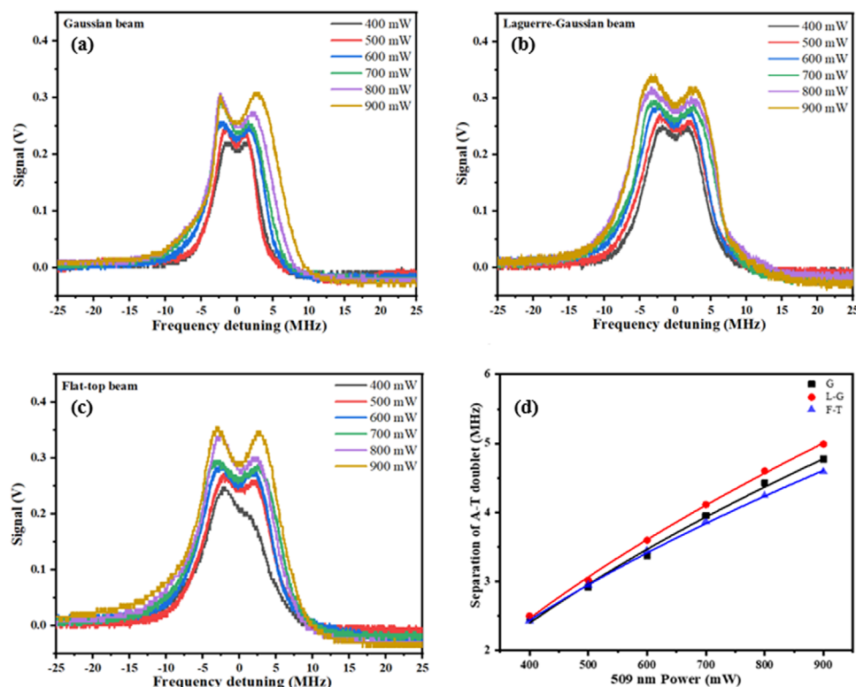
Figure 6. A-T splitting of the Rydberg EIT ( 6S_{1/2}-6P_{3/2}-5D_{5/2} ), A-T splitting distance increases with increasing coupling beam power, and the A-T splitting is utilized to calibrate the Rabi frequency. a) A-T splitting spectrum of the 509 nm for TEM 00 -mode Gaussian beam. b) A-T splitting spectrum of the 509 nm for Laguerre–Gaussian beam. c) A-T splitting spectrum of the 509 nm for flat-top beam. d) The A-T splitting interval as a function of power for three beams with different radial intensity distributions.
