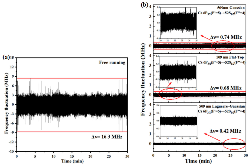
Figure 9. The frequency fluctuation of the 509 nm laser before and after being locked to 6P_{3/2}(F'=5) \rightarrow 52S_{1/2}(F''=4) Rydberg transition via TCPS scheme. a) Typical frequency fluctuation of the 509-nm laser in the free running case is about 16.3 MHz. b) The 509-nm laser is locked to the TCPS with TEM 00 -mode Gaussian, flat-top, and Laguerre–Gaussian coupling beams, respectively. The corresponding residual frequency fluctuations in 30 min are 0.74, 0.68, and 0.42 MHz, respectively. The larger the slope of TCPS resonance, the better the 510-nm coupling laser frequency stability after being locked.
