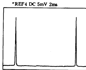
Fig. 6 The transmission of SHG output through the scanning confocal F-P cavity with a free spectral range of 750 MHz
