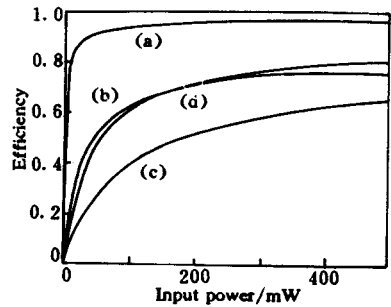
Fig. 2 Conversion efficiency as a function of the IR input power
