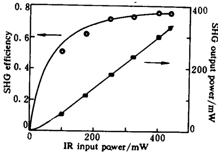
Fig. 4 SHG output power and conversion efficiency as a function of the IR input power. Circles, and squares: data; lines: theory
