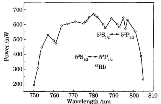
图8 钛宝石激光器输出功率随波长变化的关系曲线 Fig. 8 Tuning curve for the single-frequency CW Ti:sapphire laser
