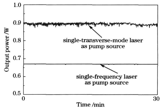
图7 钛宝石激光器30 min内的输出功率稳定性曲线 Fig. 7 Power fluctuation of the CW Ti:sapphire laser in 30 min
