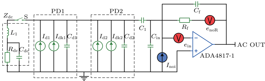
Fig. 2. The AC output noise response model of the photodetector. Some parameters are as follows: I_{\text{noi}} = 2.5 \text{ fA}/\sqrt{\text{Hz}} , I_{\text{dk1}} = I_{\text{dk2}} = 0.3 \text{ nA} , C_{\text{d1}} = C_{\text{d2}} = 5 \text{ pF} , and C_{\text{in}} = 1.4 \text{ pF} .
