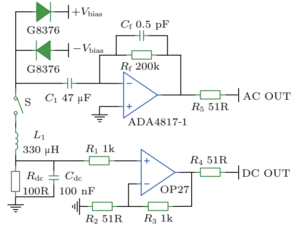
Fig. 1. The schematic of the BHD with L - C coupling and TIA circuit.
